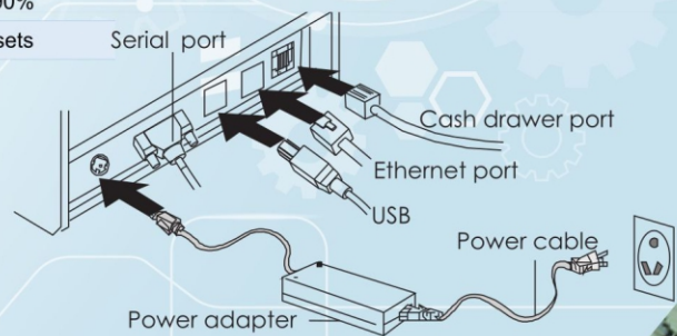
Printer connection diagram:
